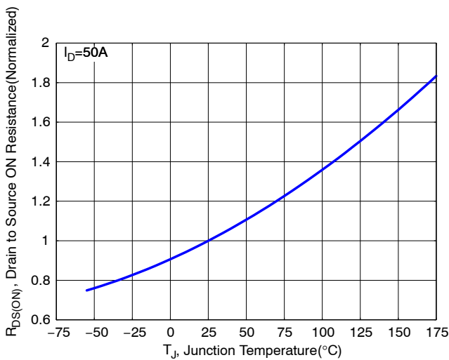
Figure 5. Normalized ON Resistance vs. Junction Temperature
