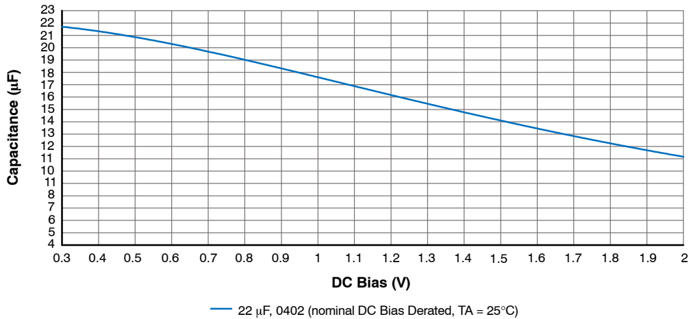
Figure 35. Typical 22 \mu\text{F} Ceramic Capacitor Value vs. DC Bias Voltage
