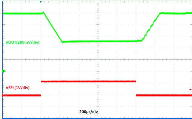
Figure 22. Vsel Toggle, V_{OUT} = 1\text{ V} to 0.5\text{ V} to 1\text{ V} , No Load, [DVS_FCCM] = 1
