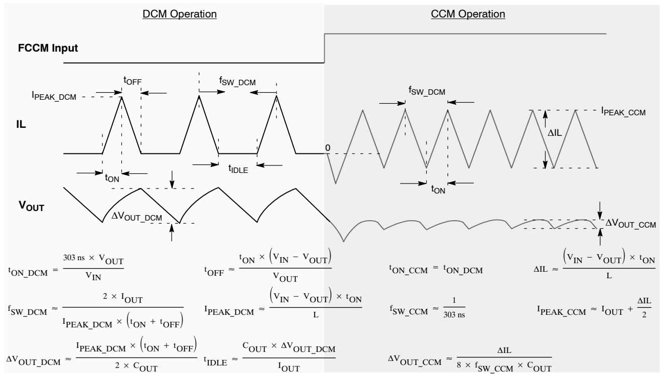
Figure 33. DCM vs. CCM Operation
