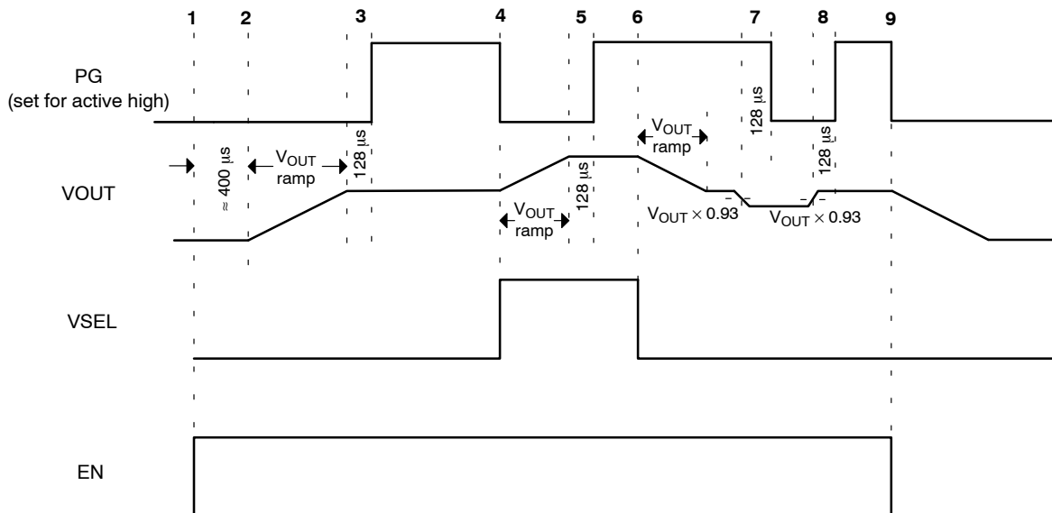
Figure 25. PG Operation
