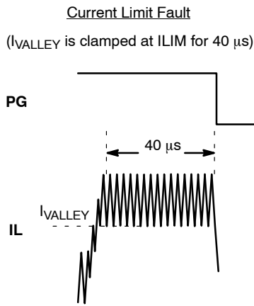
Figure 26. Current Limit Fault
