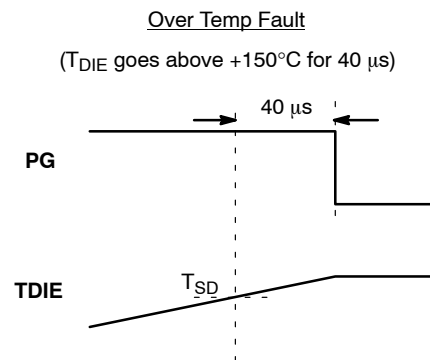
Figure 29. Over Temperature Fault
