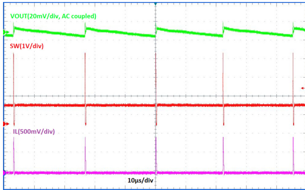
Figure 24. Device Switching (DCM), I_{OUT} = 10\text{ mA}
