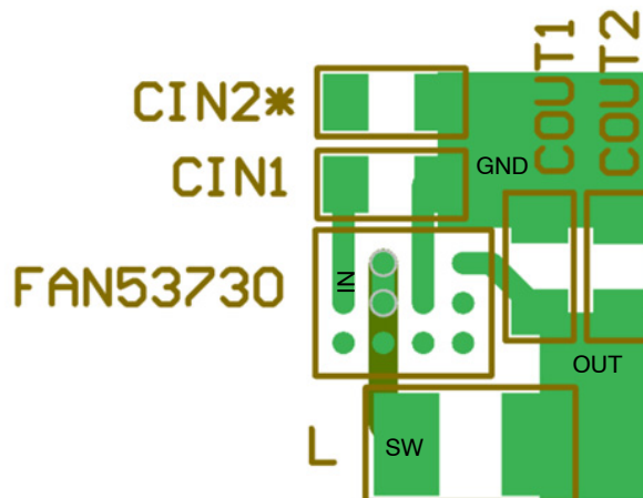
Figure 36. Layout Example
