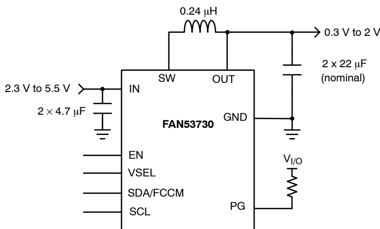
Figure 34. Typical Application Circuit
