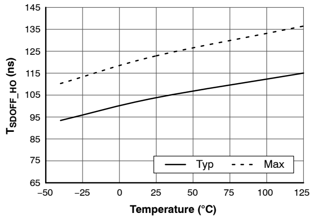
Figure 33. \overline{SD} to High-side Propagation Delay vs. Temperature
